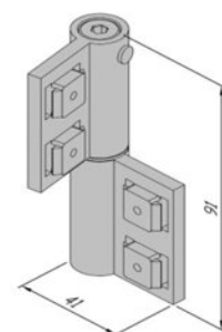
RT 50
