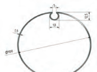
100 mm
